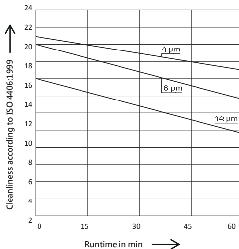
B 12µm GSEPRO® MAX 2 filter element Reference oil volume with Q_{\text{off-line filter}}=15 \text{ l/min} .
